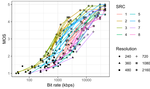
Fig. 2 Relationship between MOS and bit rate.
