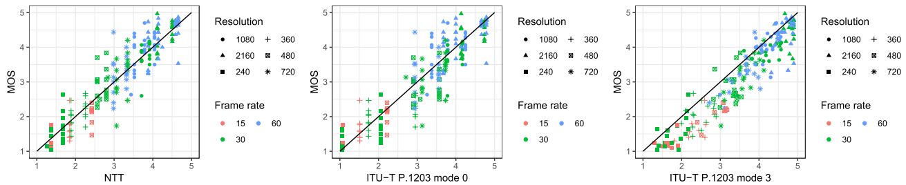
Fig. 5 Validation performance: NTT (left), P.1203 mode 0 (center), mode 3 (right).
