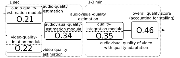
Fig. 1 General flow of audiovisual-quality estimation.
