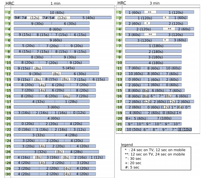
Fig. 6 Quality adaptation in long-term evaluations.
