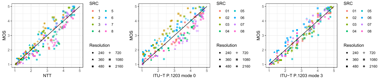
Fig. 3 Training performance - NTT (left), P.1203 mode 0 (center), mode 3 (right).
