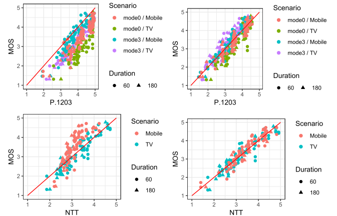
Fig. 7 Performance results. ITU-T P.1203 (top), NTT (bottom). Transferred coefficients (left), retrained coefficients (right).
