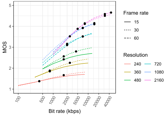
Fig. 4 Relationship between MOS and bit rate. Estimations from NTT model. Solid black circles mark selected coding conditions.
