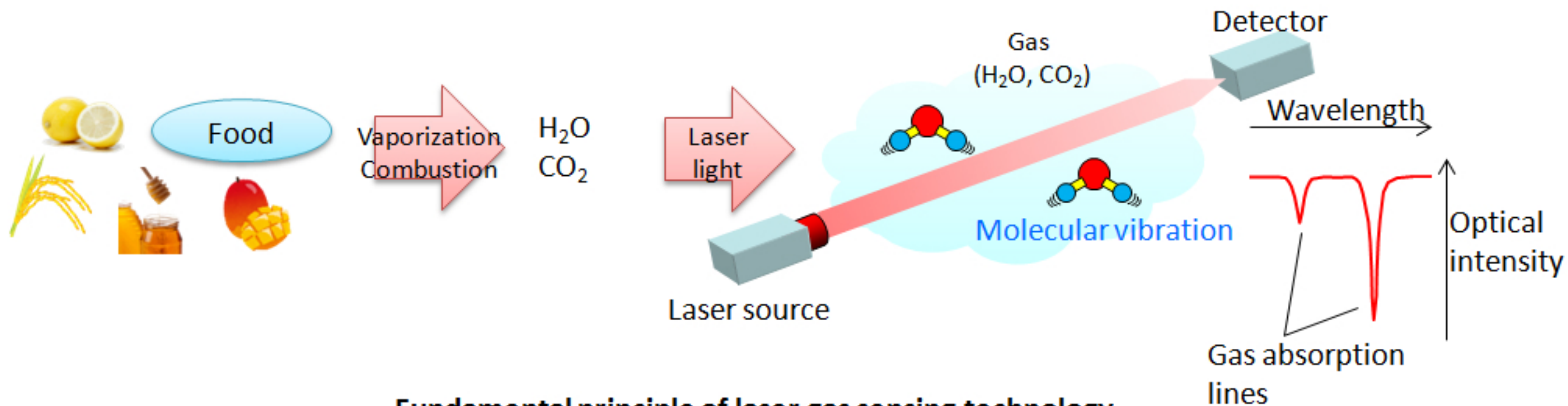
Fundamental principle of laser gas sensing technology
