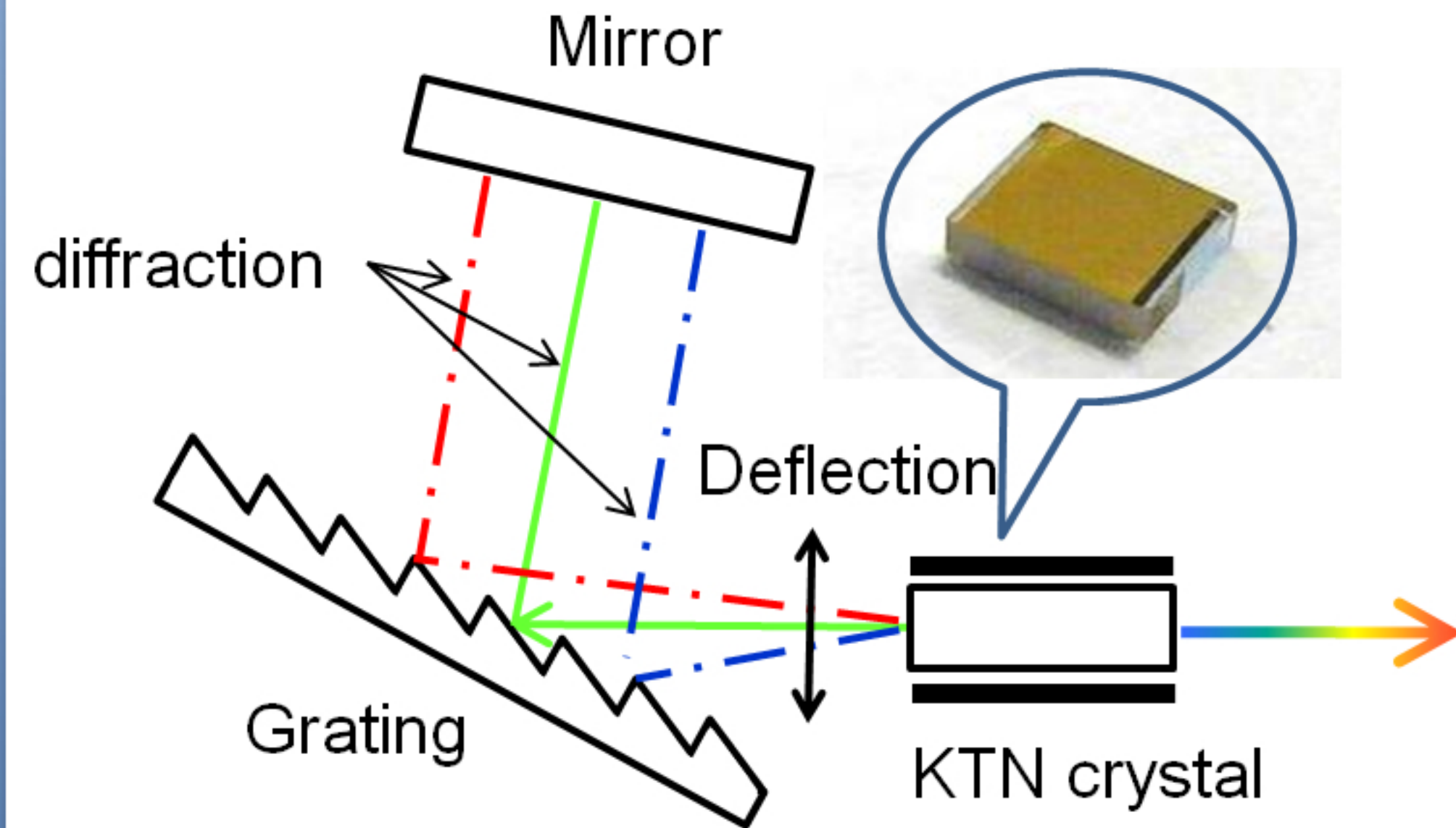
Operating principle of wavelength sweep by KTN crystal
