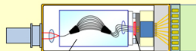
PLC demultiplexer APD Array
