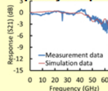
E/O Frequency Response
