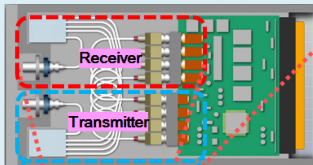
CFP Transceiver (82 x 145 mm)
