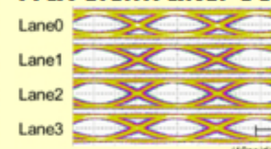
Waveform after 50-km transmission
